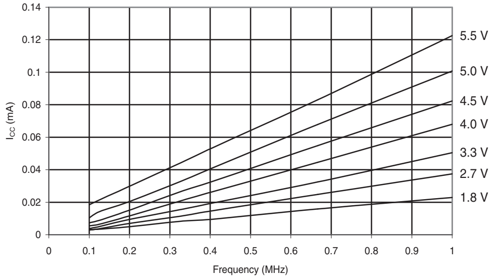
Figure 29-92. ATmega48PA: Reset Supply Current vs. Low Frequency (0.1 - 1.0 MHz)
