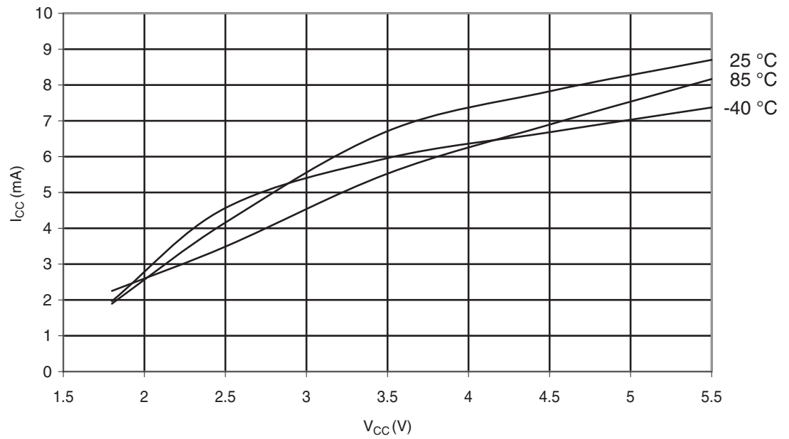
Figure 29-373. ATmega328P: Programming Current vs. V_{CC}
