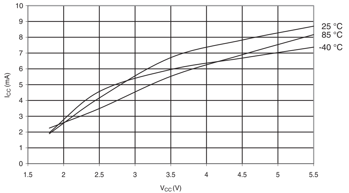
Figure 29-326. ATmega328: Programming Current vs. V_{CC}
