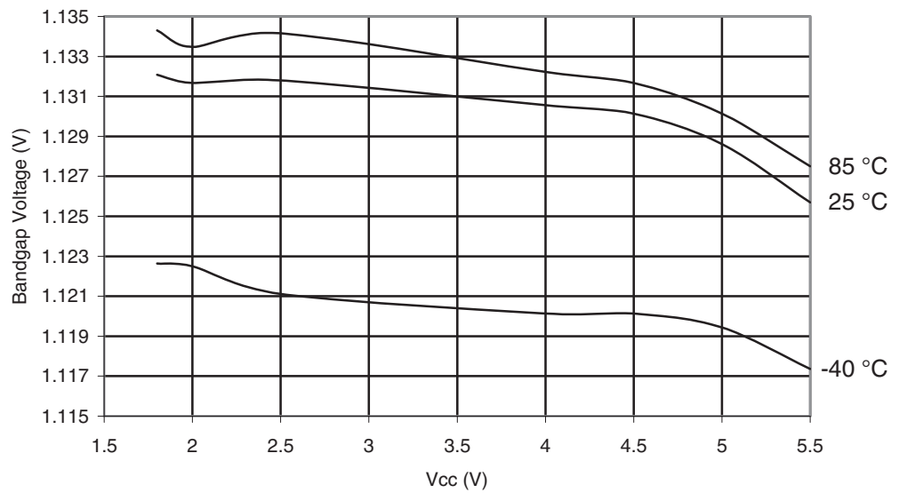
Figure 29-269. ATmega168PA: Bandgap Voltage vs. V_{CC}
