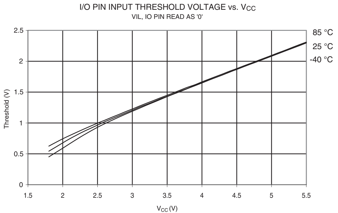
Figure 29-308. ATmega328: I/O Pin Input Threshold Voltage vs. V_{CC} ( V_{IL} , I/O Pin read as '0')
