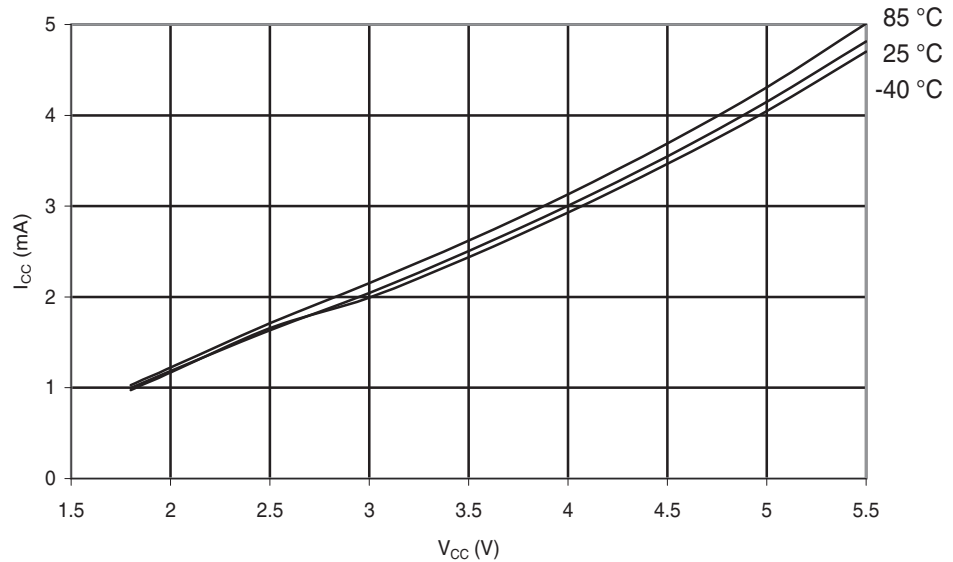
Figure 29-240. ATmega168PA: Active Supply Current vs. V_{CC} (Internal RC Oscillator, 8 MHz)
