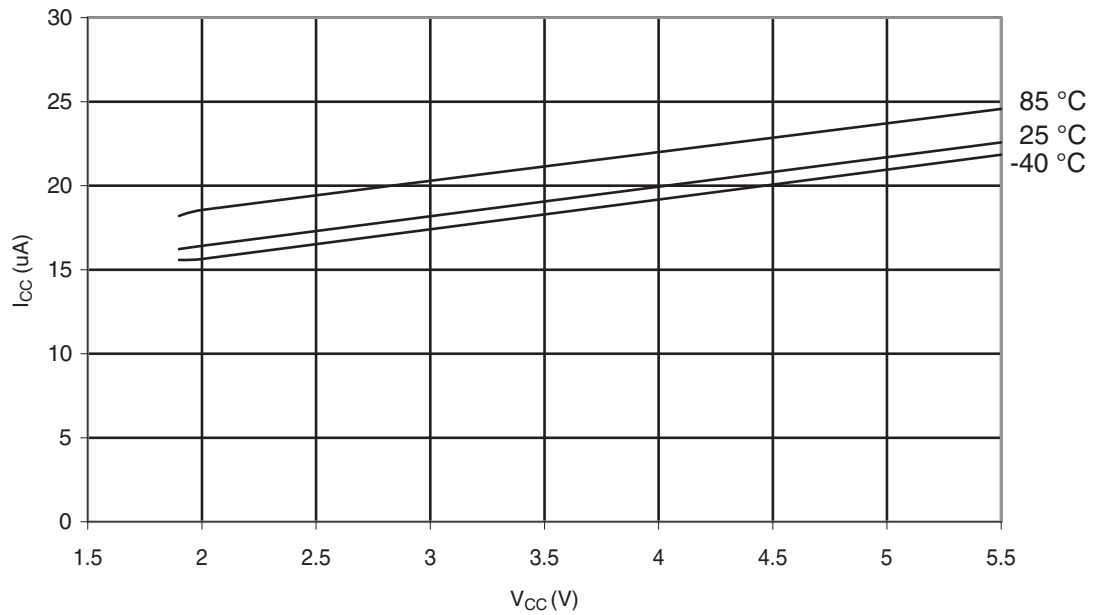
Figure 29-372. ATmega328P: Brownout Detector Current vs. V_{CC}
