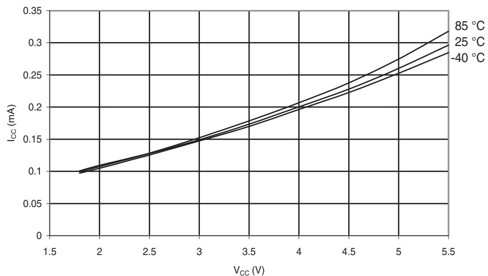
Figure 29-150. ATmega88PA: Idle Supply Current vs. V_{CC} (Internal RC Oscillator, 1 MHz)
