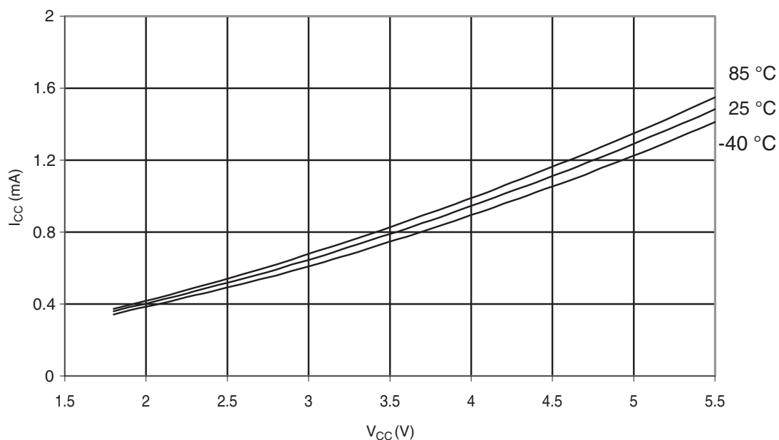
Figure 29-292. ATmega328: Idle Supply Current vs. V CC (Internal RC Oscillator, 8 MHz)
