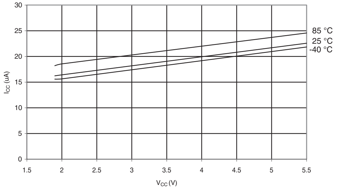
Figure 29-325. ATmega328: Brownout Detector Current vs. V_{CC}
