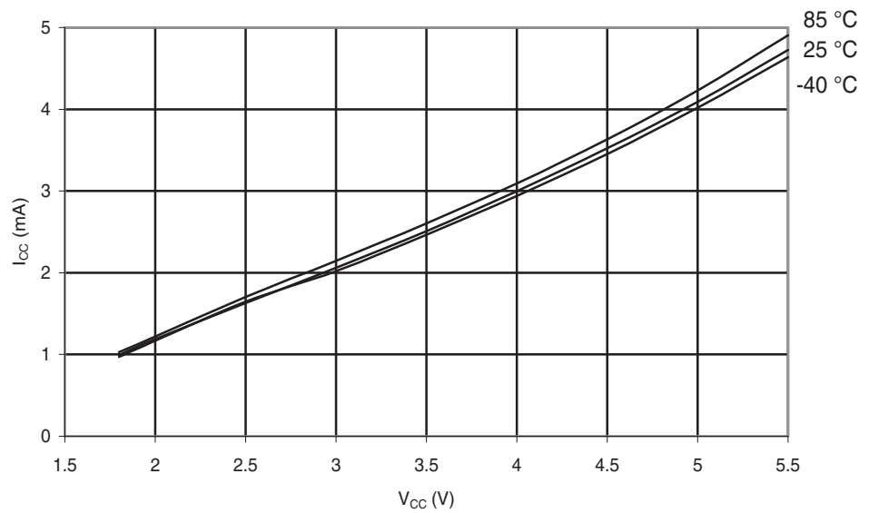
Figure 29-146. ATmega88PA: Active Supply Current vs. V_{CC} (Internal RC Oscillator, 8 MHz)
