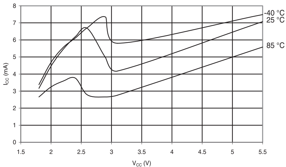
Figure 29-185. ATmega88PA: Programming Current vs. V_{CC}
