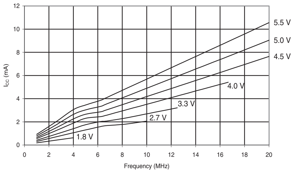
Figure 29-190. ATmega168A: Active Supply Current vs. Frequency (1-20 MHz)
